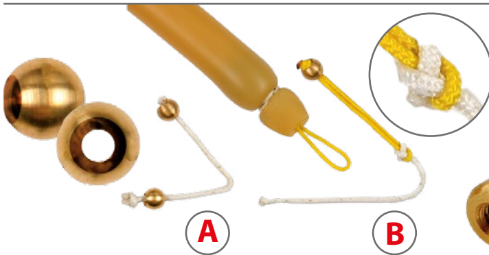
Item 023004001 Small brass perforated binding rings \varnothing 8 mm. for Dyneema® ogives, either simple (A) or interchangeable (B)
